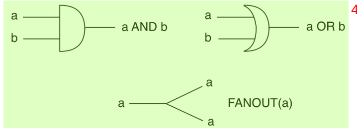
Fig. 3.1 Classical gates 5
