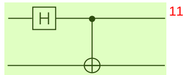
Fig. 3.3 Entangler gate, produces the Bell states 12
