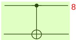
Fig. 3.2 CNOT gate 9
