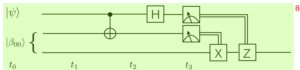
Fig. 4.1 Teleportation circuit 9
