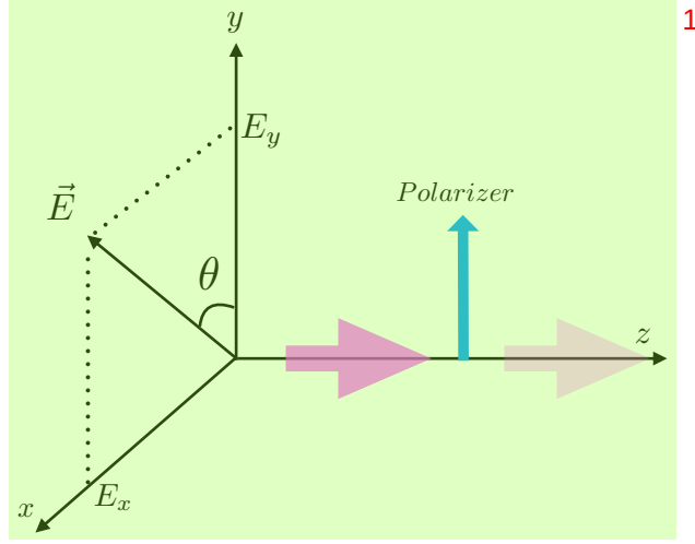
Fig. 1.3 Polarized radiation 2
